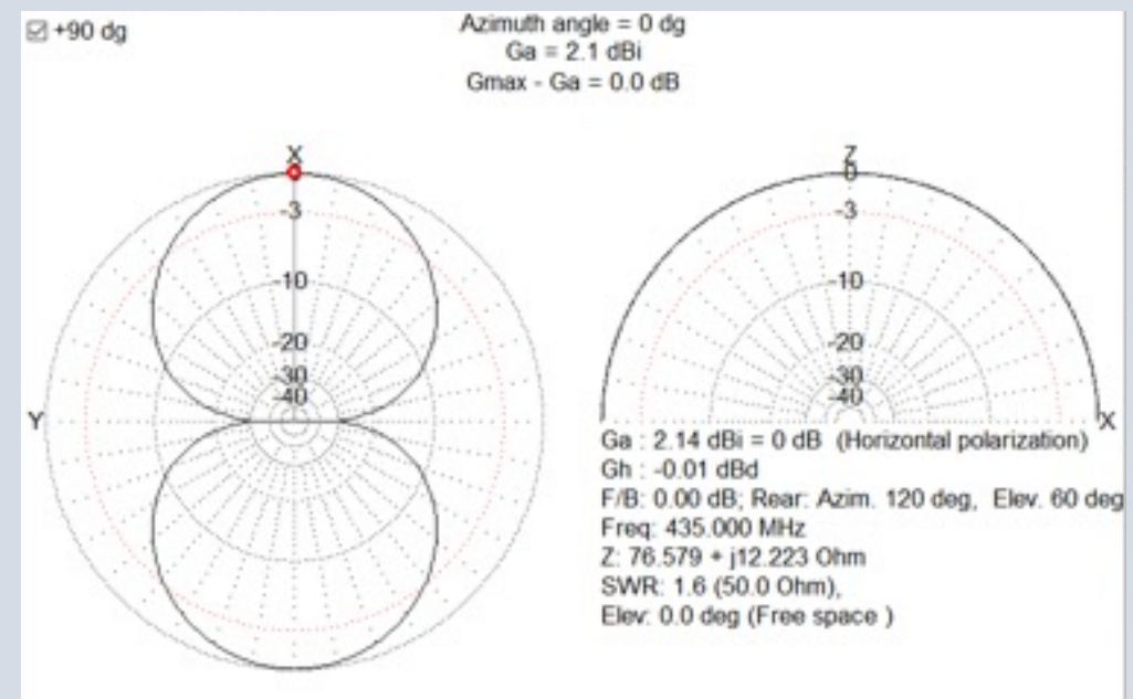
2D Radiation Pattern (Directivity)
