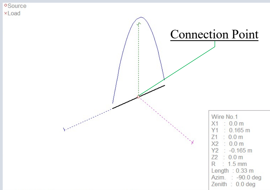
Structure of UHF DP Antenna
