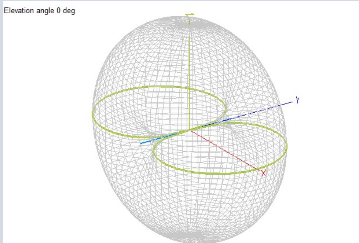
3D Radiation Pattern (Directivity)
